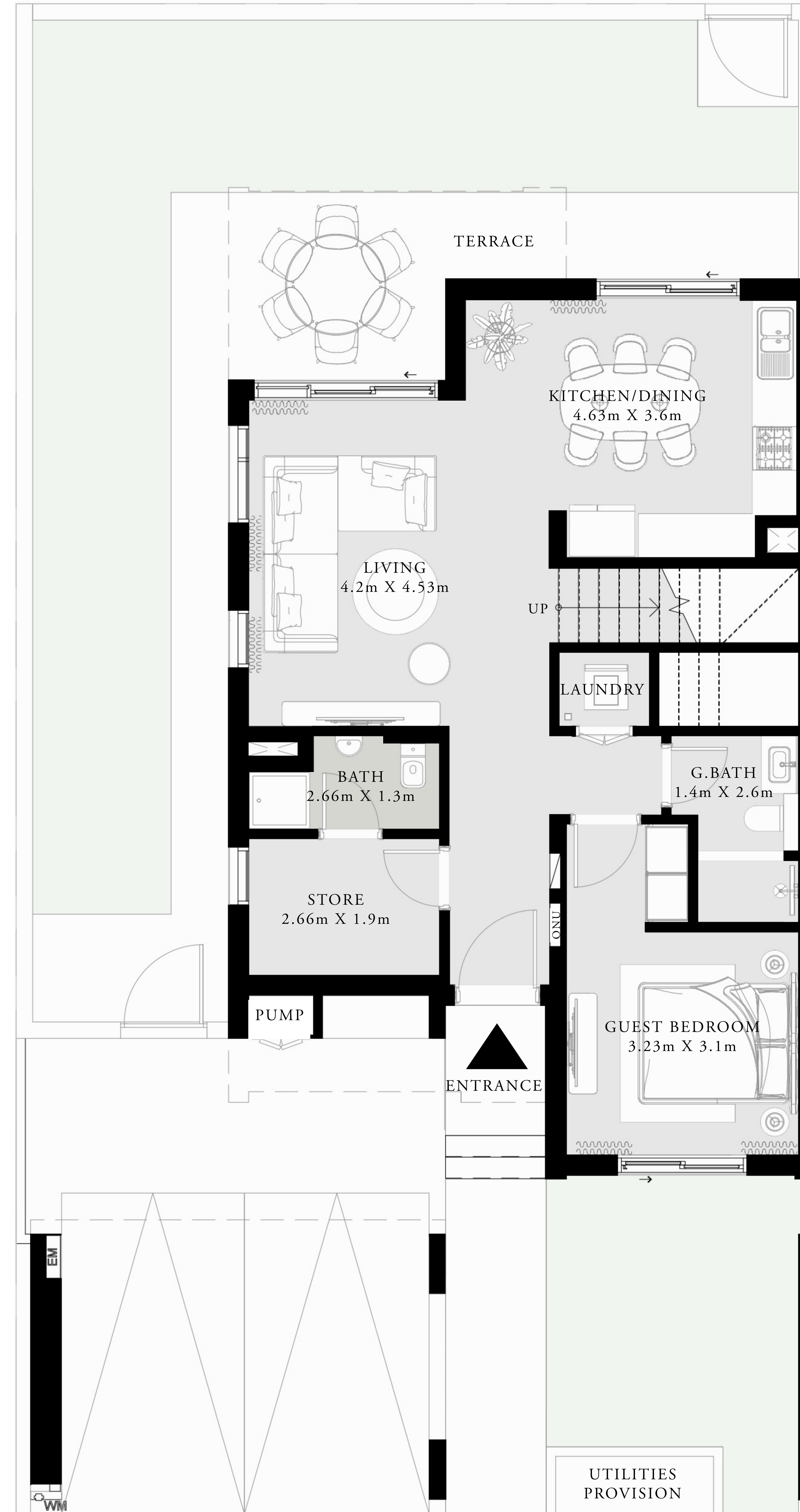
GROUND FLOOR
