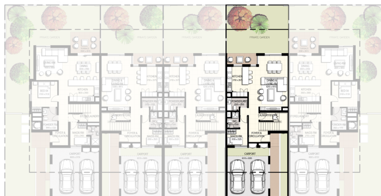
5 unit cluster
