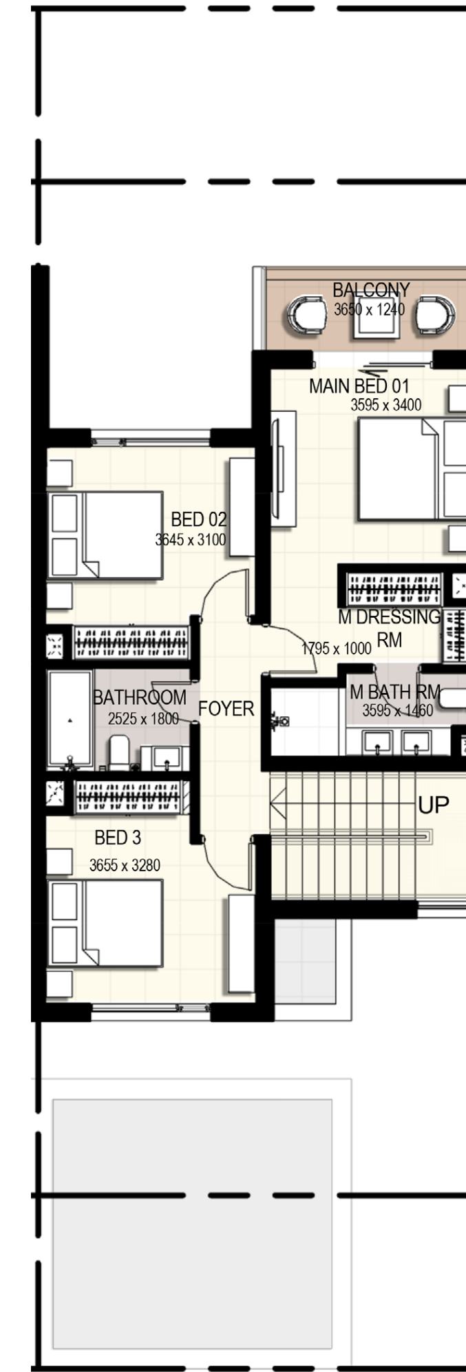
First Floor
