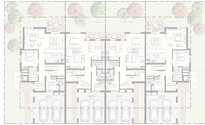
4 unit cluster
