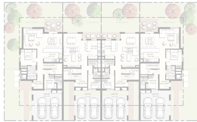
4 unit cluster
